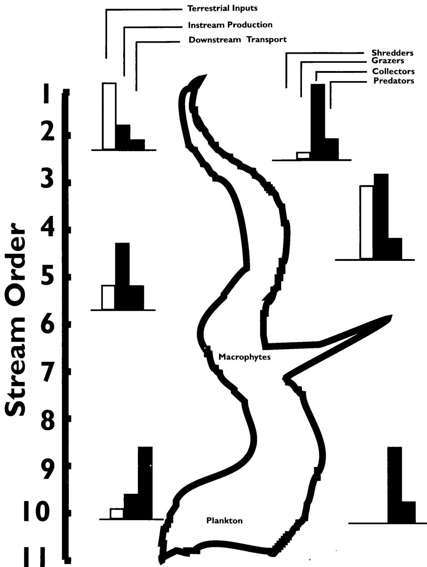
Figure 1. Schematic of the river-continuum concept depicting the river channel from first order to large river (After Johnson et al. 1995).
