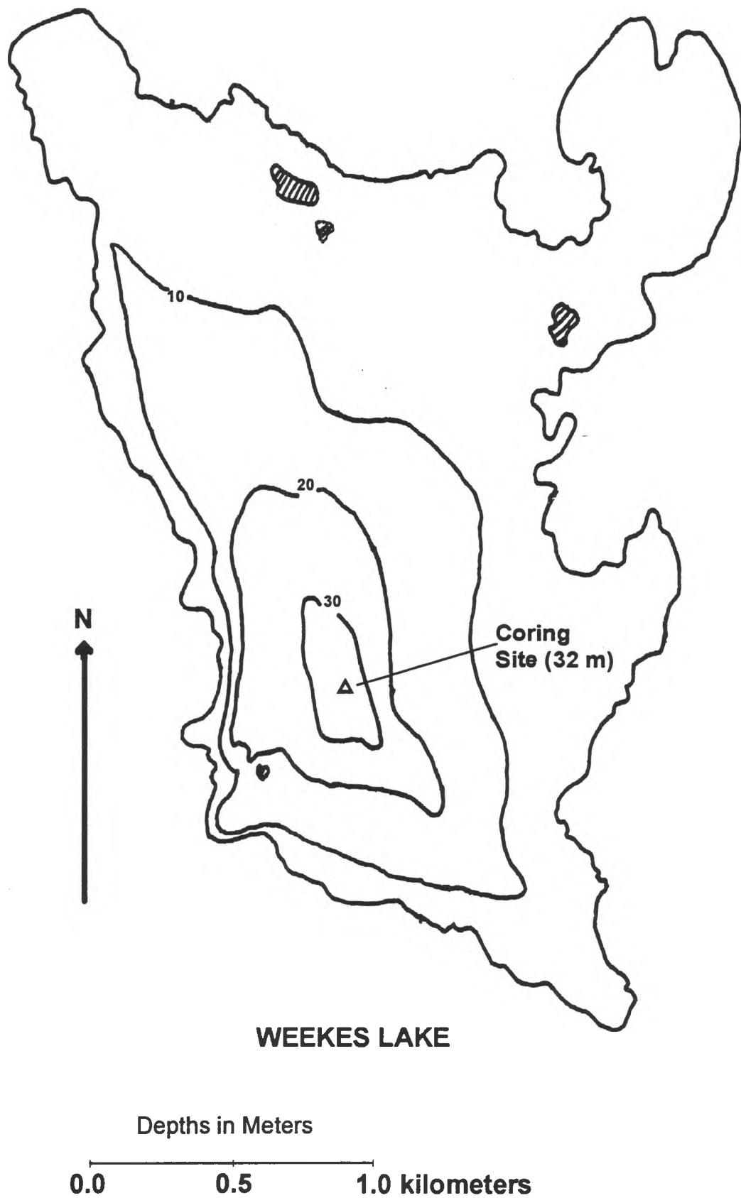
Figure 3: Bathymetric Map of Weekes Lake.
