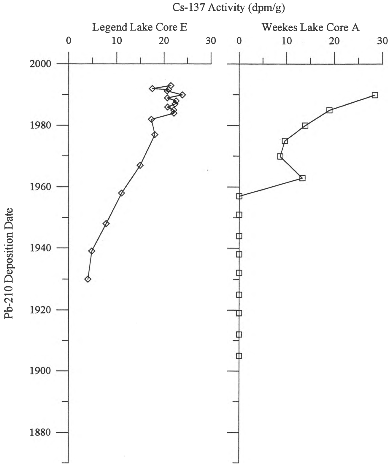
Figure 9: Cs-137 Activity Plotted Against Pb-210 Dates. Legend and Weekes Lakes.
